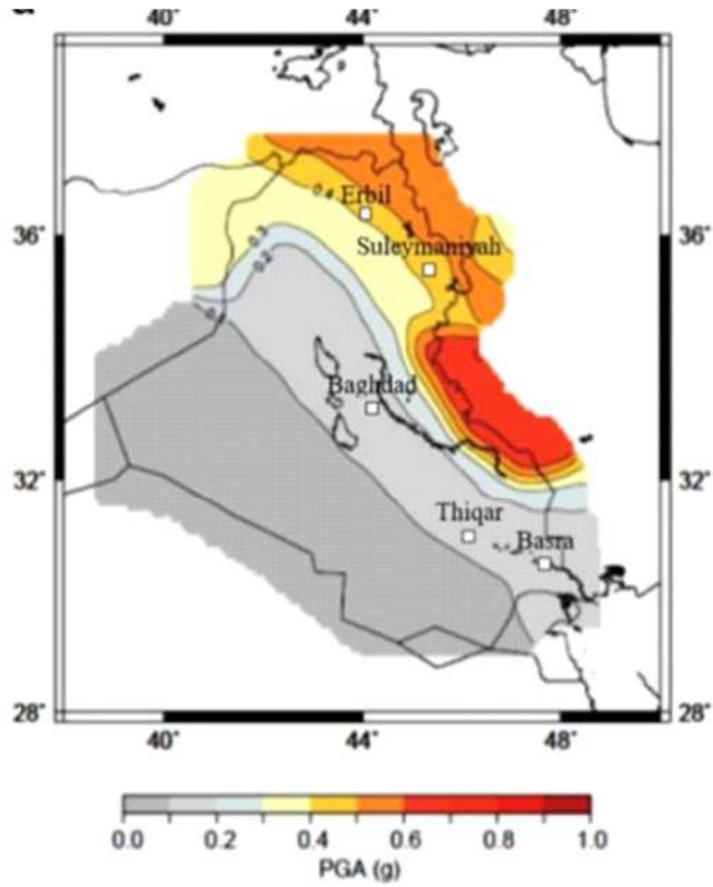
Seismic Hazard Map of Iraq
