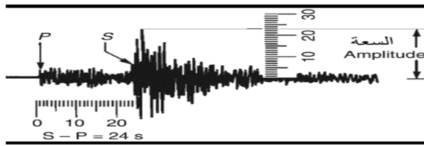
Measuring of ground motion amplitude on seismogram
